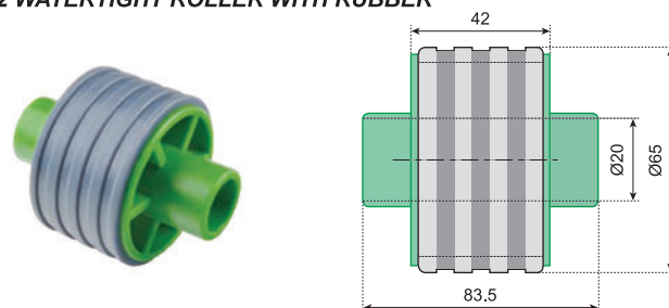
N452 WATERTIGHT ROLLER WITH RUBBER
