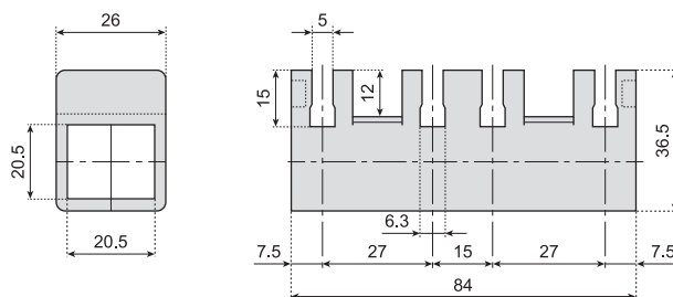
N486 SPACER FOR SERPENTINE
