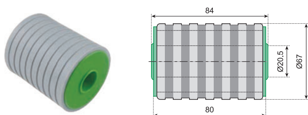
N453 WATERTIGHT ROLLER WITH RUBBER
