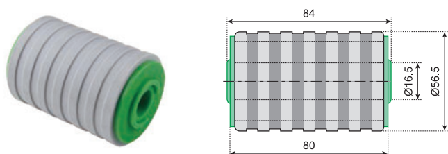
N454 WATERTIGHT ROLLER WITH RUBBER
