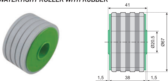
N451 WATERTIGHT ROLLER WITH RUBBER
